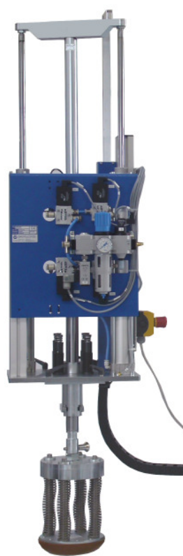
Installation set drop tester for universal test fields order no.: 41-013-218
