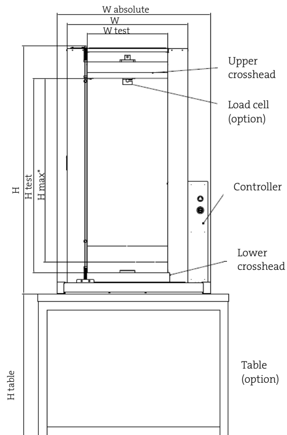
View universal testing machine with dimensions
