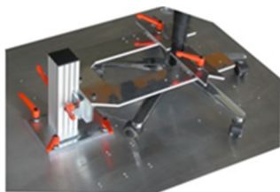
40-001-115 Universal holding device for foot rests of seating furniture; height adjustable
