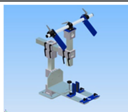
40-001-095 Universal holding device for foot rests; height adjustable, extended for rotary tests
